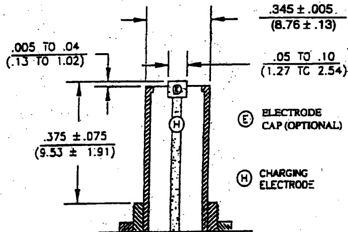
CHARGING PEDESTAL
